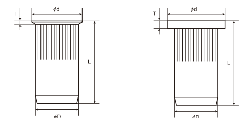
NSK-□MR (Small flange) NSD-□MR (Large flange)
