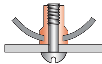
Fastening piping to flat board
