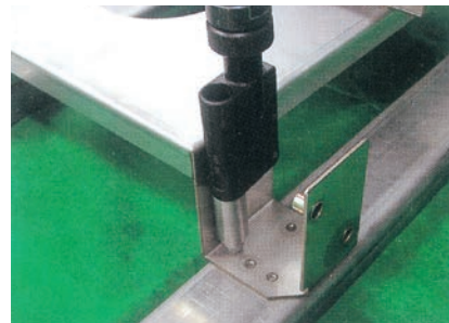
00 Offset nose of AR2000A-00 allows perfect riveting at dead set place
